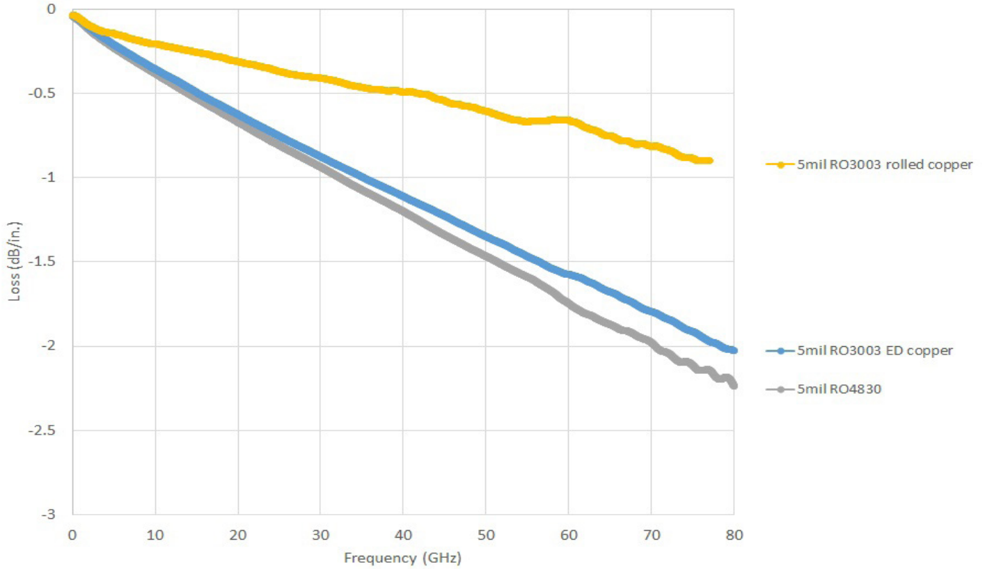
Microstrip insertion loss, differential length method using 5mil and 9.4mil RO4830™ laminate and 5mil RO3003™ laminate
