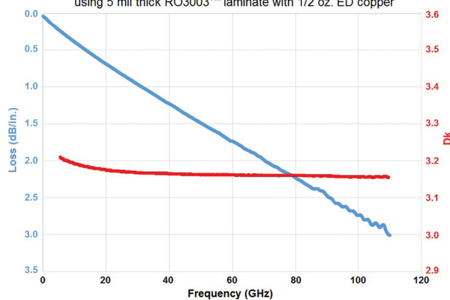
Very wideband insertion loss & phase measurements
