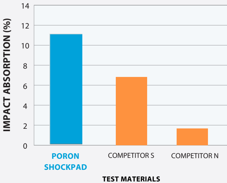
GRAPH 1: IMPACT PROTECTION: 0.10MM FOAM
