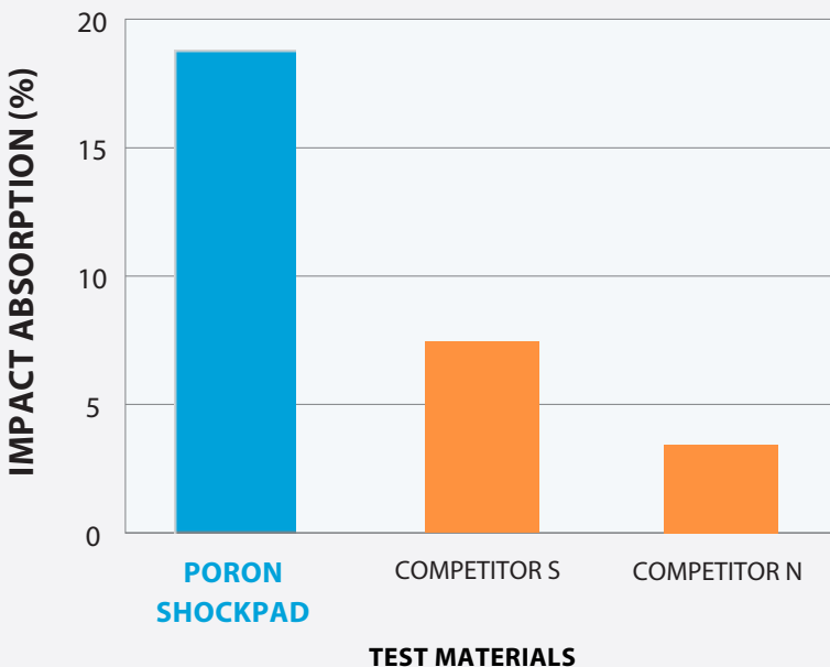
GRAPH 2: IMPACT PROTECTION: 0.15MM FOAM
